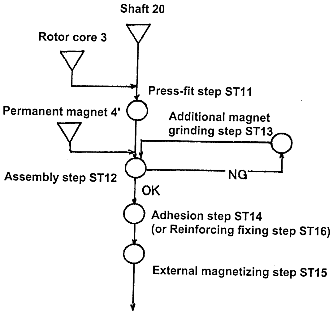
Fig. 14 (Prior Art)
